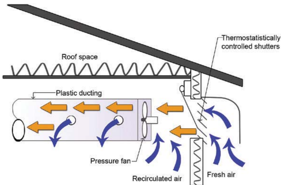
Figure 6.3: Ducting Fitted
