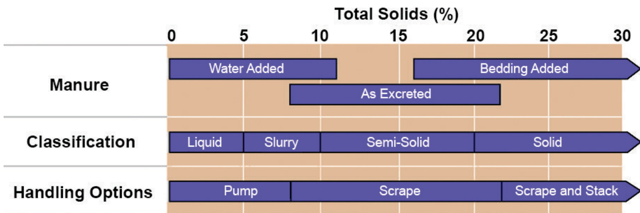
Figure 1.1: Total Solids and Manure Handling Options
