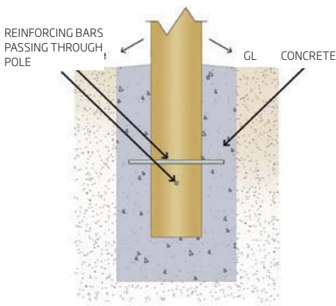
Figure 5.3: Timber Pole Base Detail
