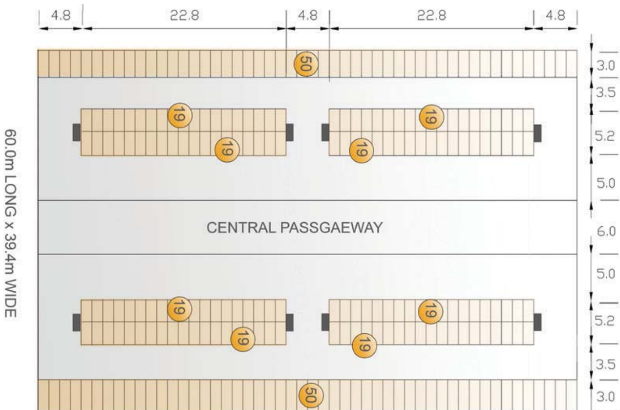
Figure 2.4: Three Row Stall System with Central Passageway 252 stalls in 2 groups of 126, suitable to house 240 cows (5% additional stalls)
