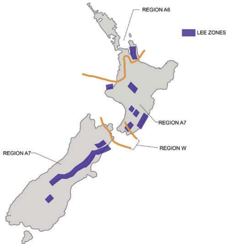
Figure 2.1: Wind Regions (illustrative only and may be subject to future change) Adapted from AS/NZS 1170.2: 2011 Fig 3.1(B))
