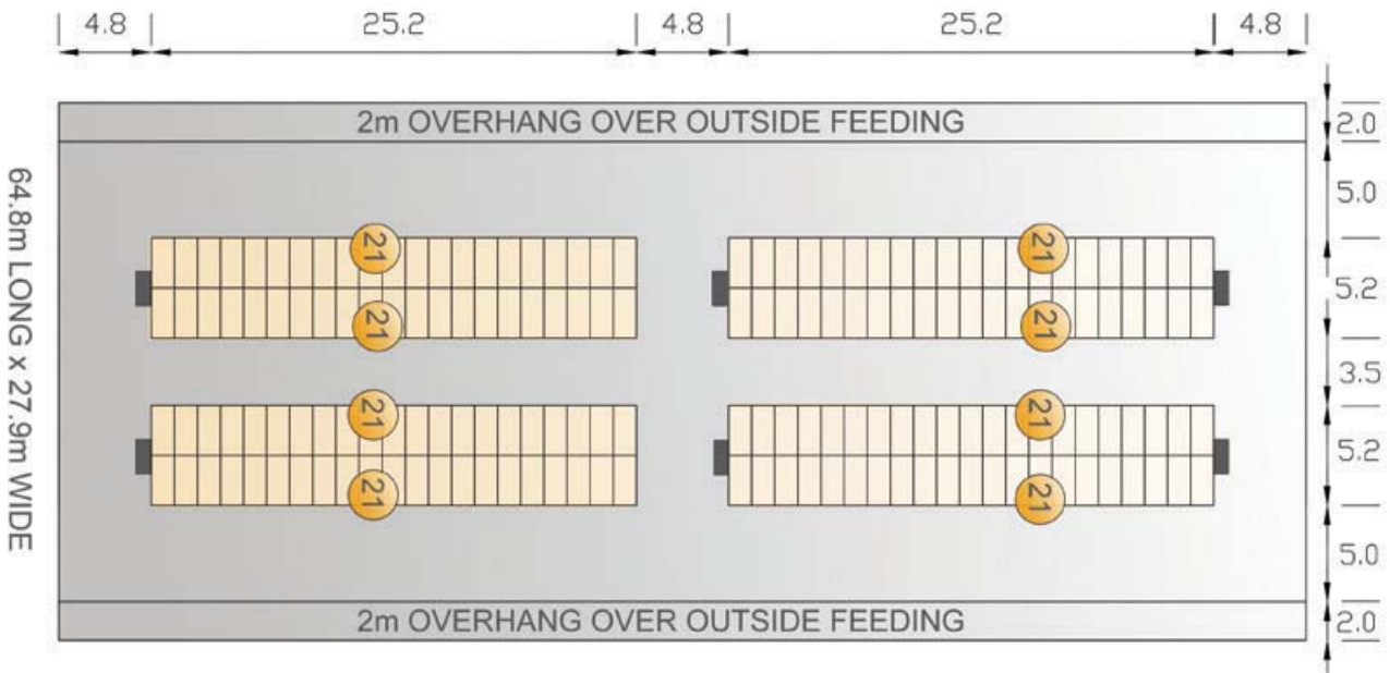
Figure 2.6: Two Row System with Outside Feeding 168 stalls in 1 group, suitable to house 160 cows (5% additional cubicles)
