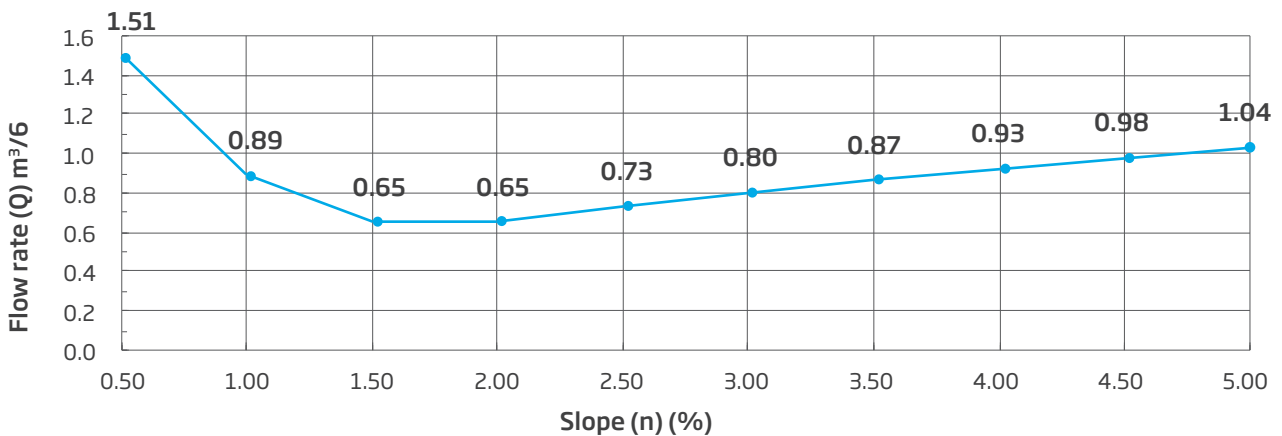
Figure 4.1: Flow Rate (m 3 /s) Required to Flush a 12-metre-wide Yard
