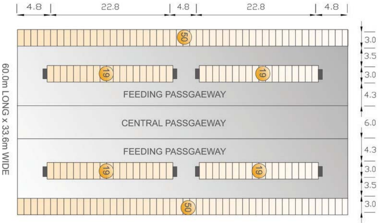
Figure 2.5: Two Row System with a Central Passageway 176 stalls in 2 groups of 88, suitable to house 167 cows (5% additional stalls)
