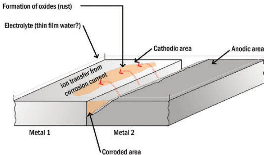
Figure 7.2: Galvanic Corrosion
