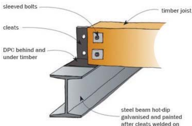
Figure 7.1: Connection of Timber to Steel
