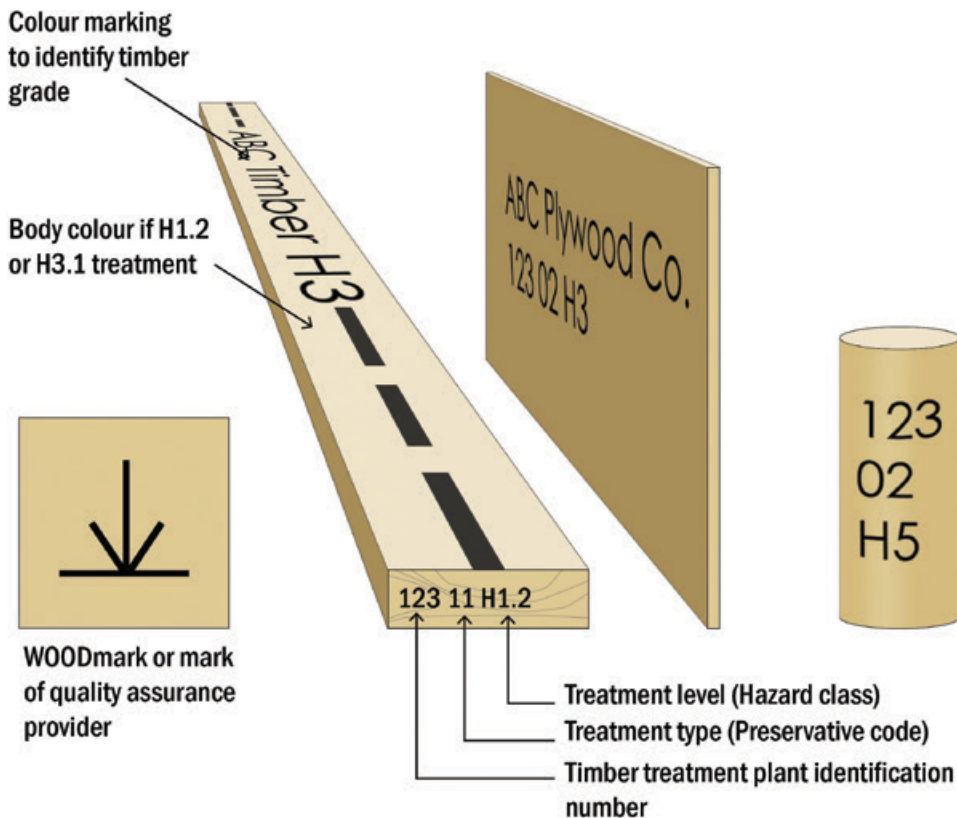
Figure 6.1: Treated Timber Branding Adapted from Figure 1 BRANZ Build 128 )
