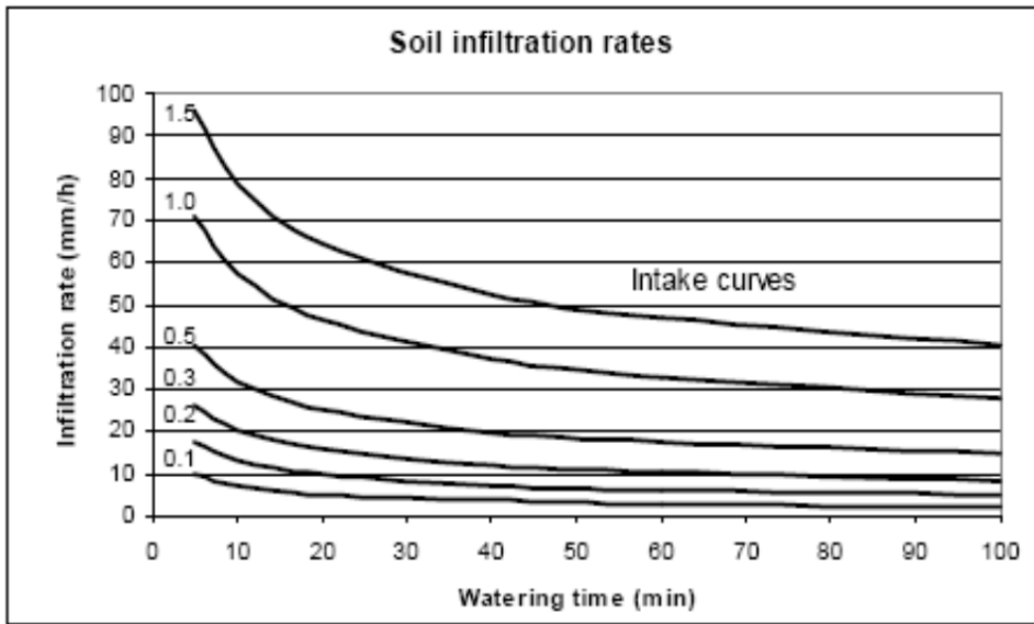
Figure 2: Soil infiltration rates according to watering time (source: INZ, 2007)
