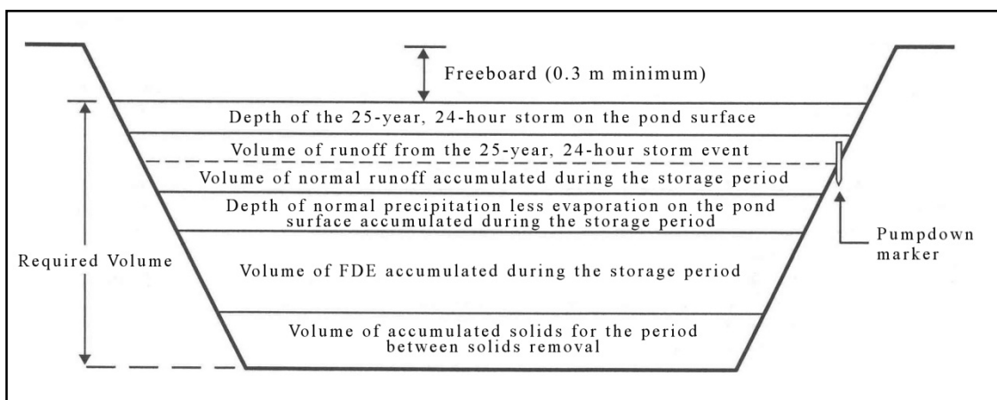
Figure 1: Cross section of liquid FDE storage pond with a watershed (modified from: USDA, 1997, Figure 10-15)
